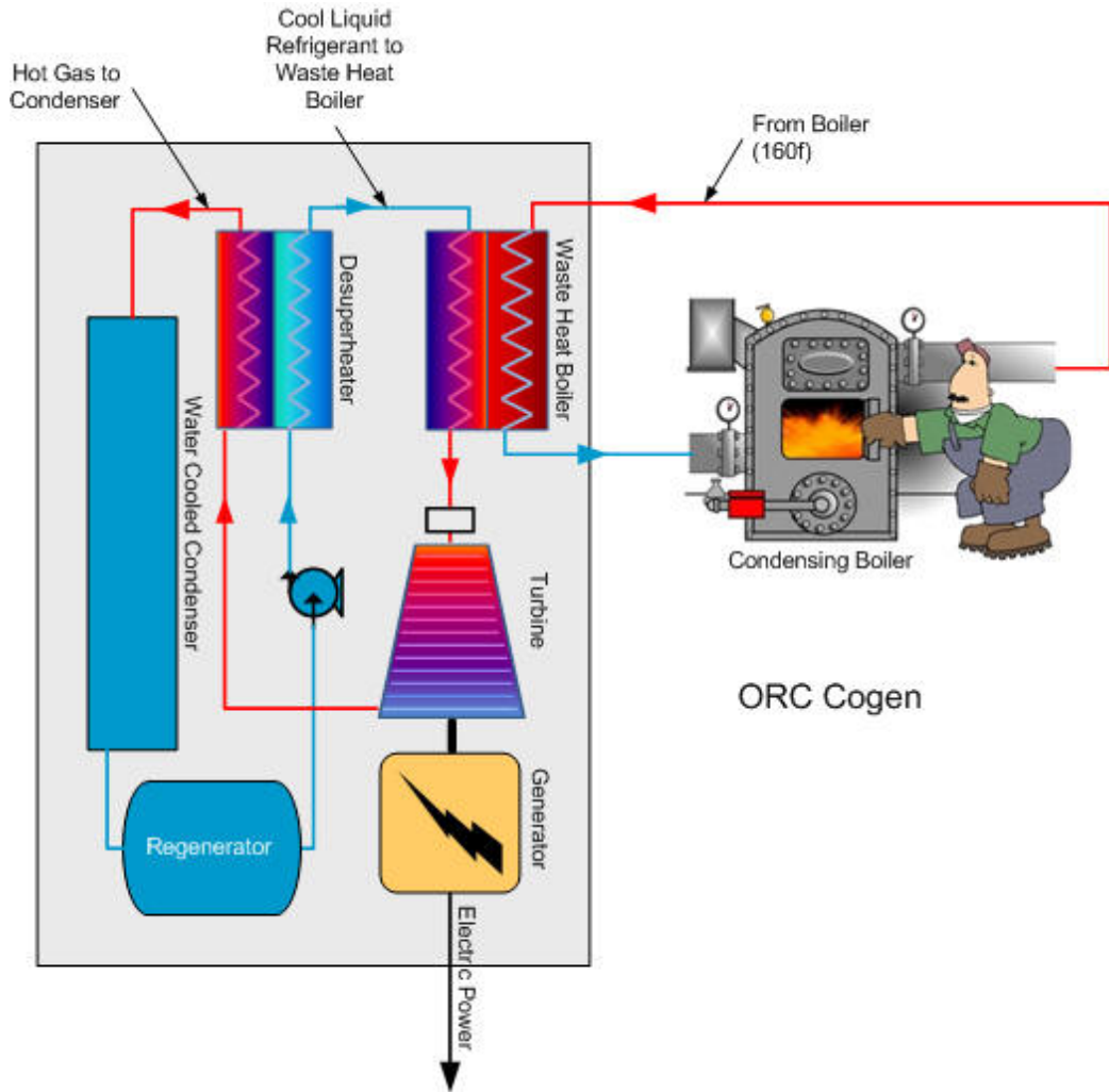
TransPacific Energy flow diagram for cogeneration heat recovery
