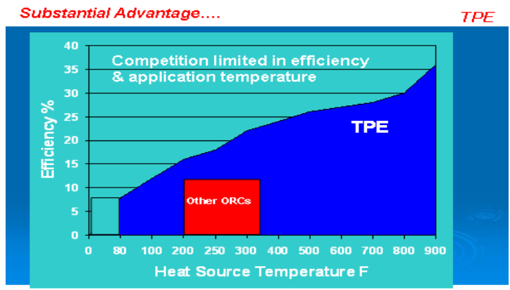
Efficiencies may vary depending upon condensation temperatures.
